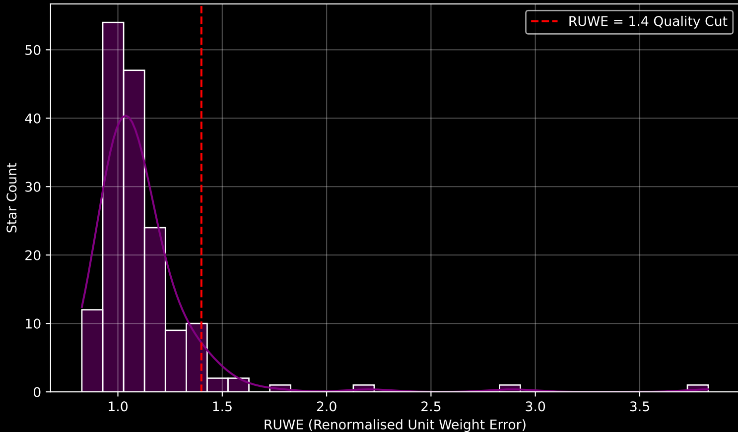
GAPOGEE DR17 Field [351+21-O] RUWE Distribution (n= 164)
