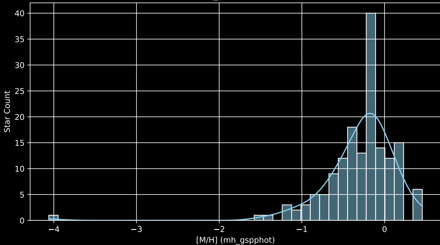
APOGEE DR17 Field: [351+21-O [M/H] (mh_gspphot) (n= 160)
