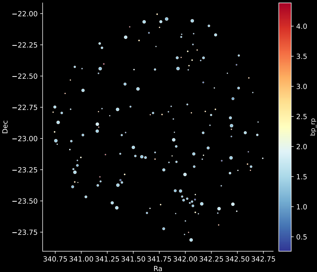
APOGEE DR17 Field: [351+21-O] Stars: 167
