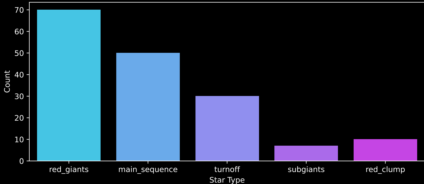
APOGEE DR17 Field: [351+21-O] Count plot of Star Type
