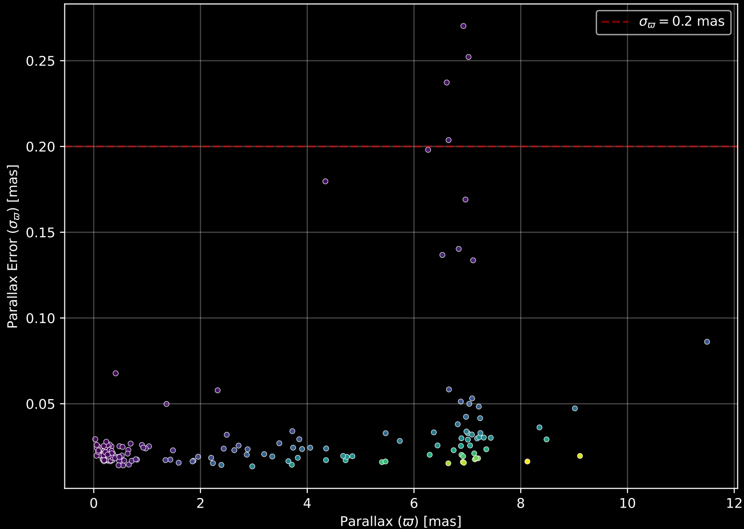
APOGEE DR17 Field: [351+21-O] Parallax Quality (n= 167)
