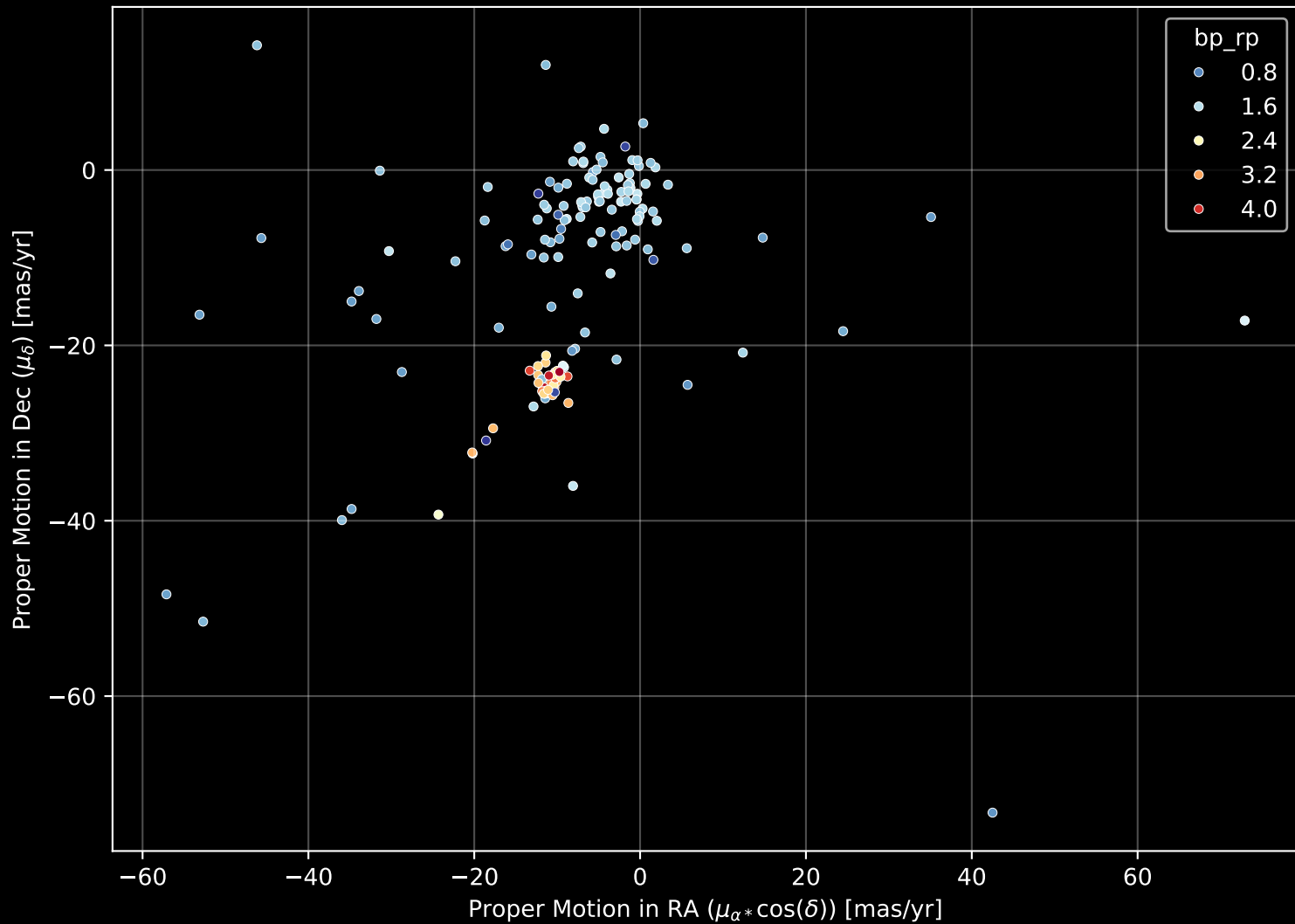
APOGEE DR17 Field: [351+21-O] Proper Motion Diagram (n= 167)
