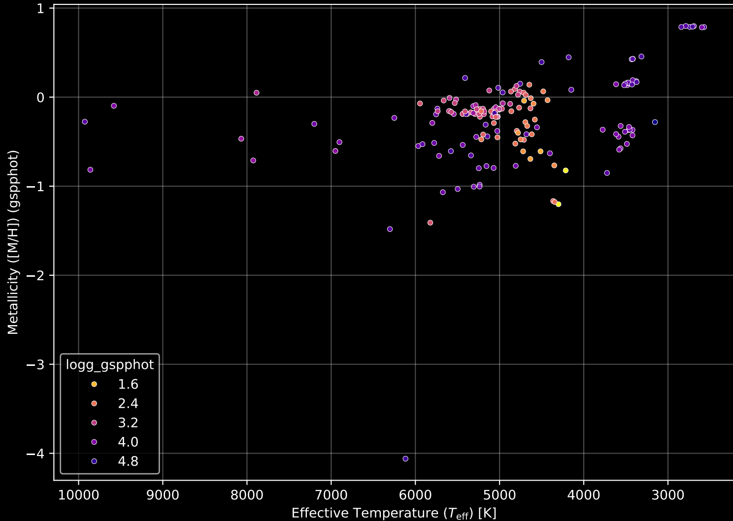
APOGEE DR17 Field: [351+21-O] Stellar Population Parameters (n= 167)
