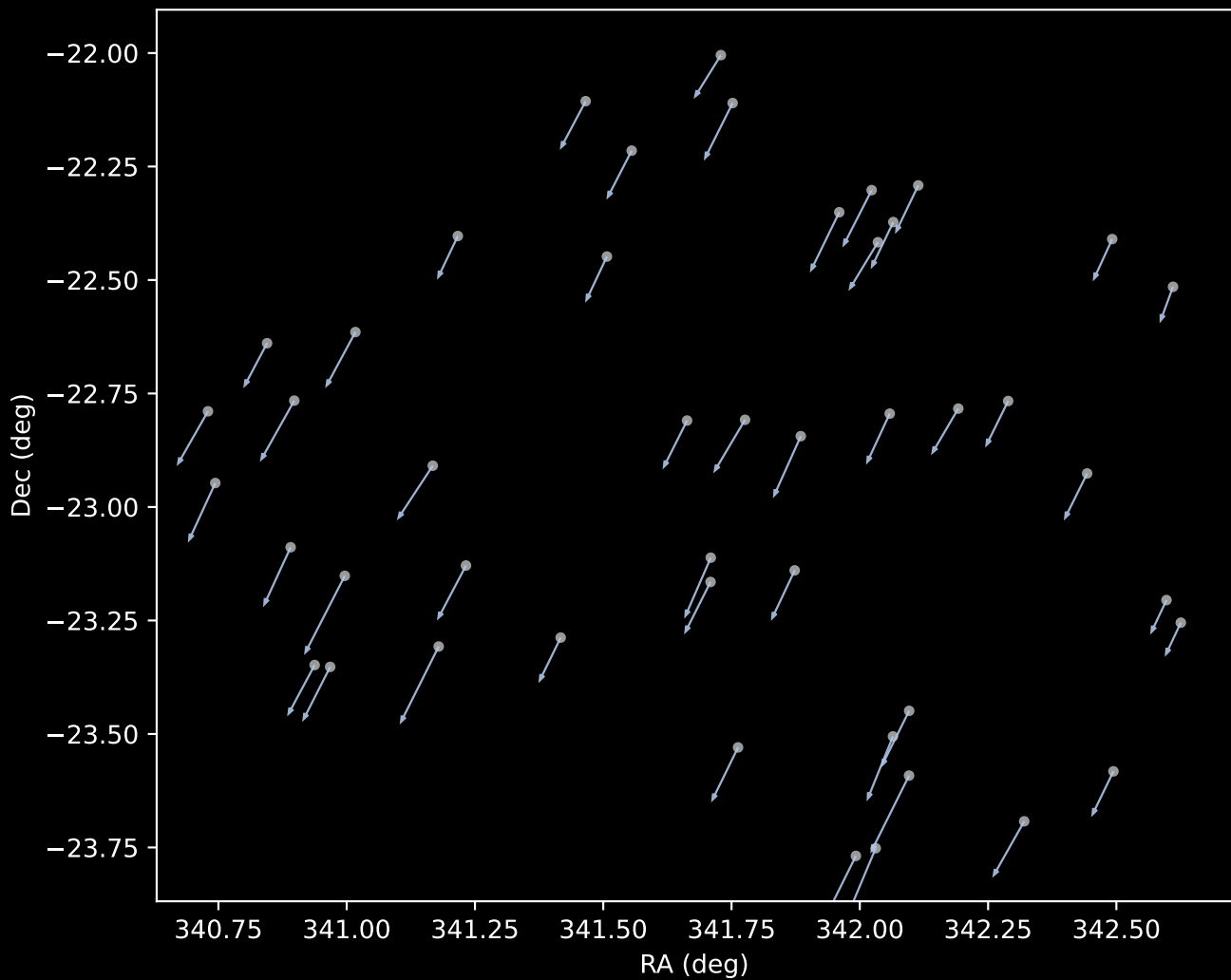
APOGEE DR17 Cluster 1 Proper Motion Vectors (n=46)
